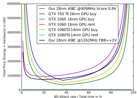
Fig. 5: Impact of the BD/NB time ratio on the cost
