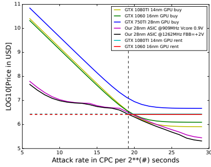
Fig. 17: Total cost (HW+E) for 100k CPC attack at a given attack rate: ASIC vs GPU
