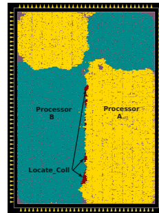
Layout Birthday core.
