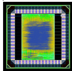
Sample 1\text{mm}^2 . asic layout with 1 NB core.
