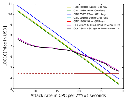
Fig. 15: CPC machine price for different attack rates: ASIC vs GPU
